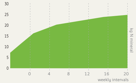
N-release at 25°C (laboratory experiment) kg N mineral / mton (accumulated)
