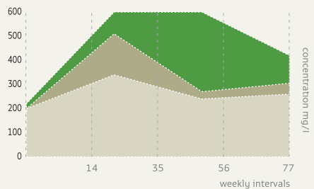
Concentration NO 3 in the top 12 cm of the soil
